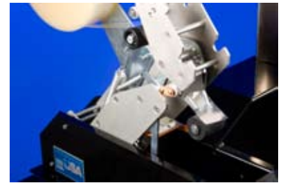
Top and bottom tape heads are interchangeable and tip back for easy threading.
