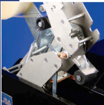
Top and bottom tape heads are interchangeable and tip back for easy threading.
