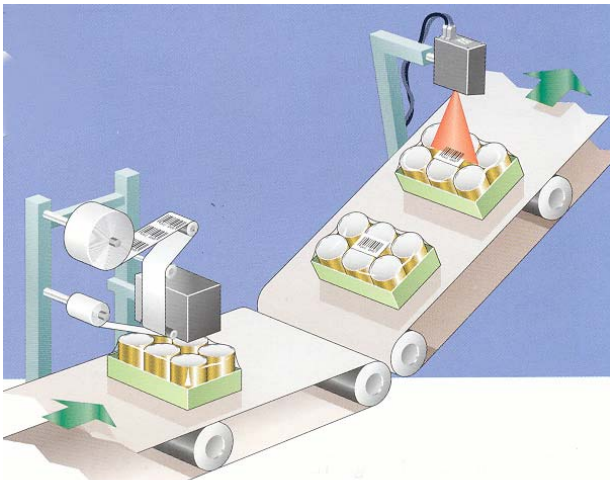
Verification or scanning after ink jet or print & apply
